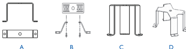
Hubodometer Bracket Types
